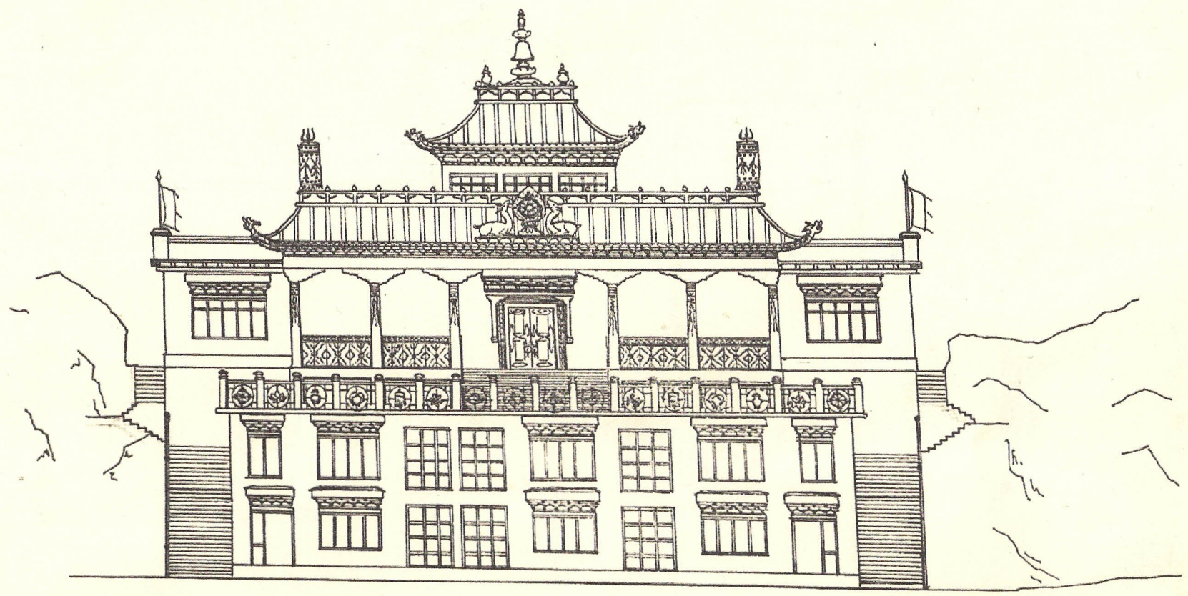
FRONT ELEVATION
